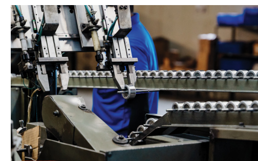
WORKSHOP 04 Produce semi-finished products "Rotor", supply to Workshop 02.
